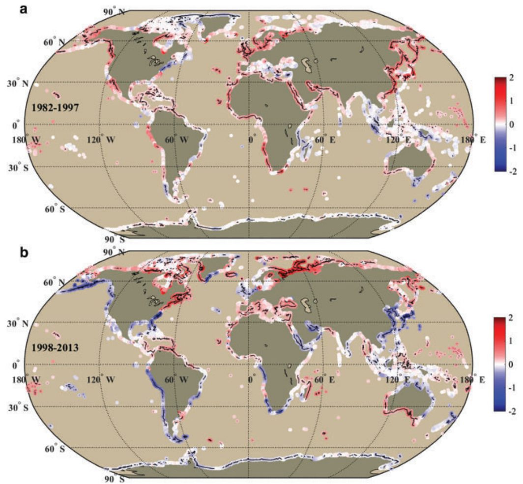
Figure 5. The linear SST trends along the world's coastlines in the warming and "hiatus" periods. The linear SST trends (unit: °C/decade) along the world's coastlines in the warming (1982–1997, a) and hiatus periods (1998–2013, b). Black points/lines in the shading color indicate that the trends in those locations are significant in statistics ( P < 0.05 ). Cited from Liao et al. [2015].
