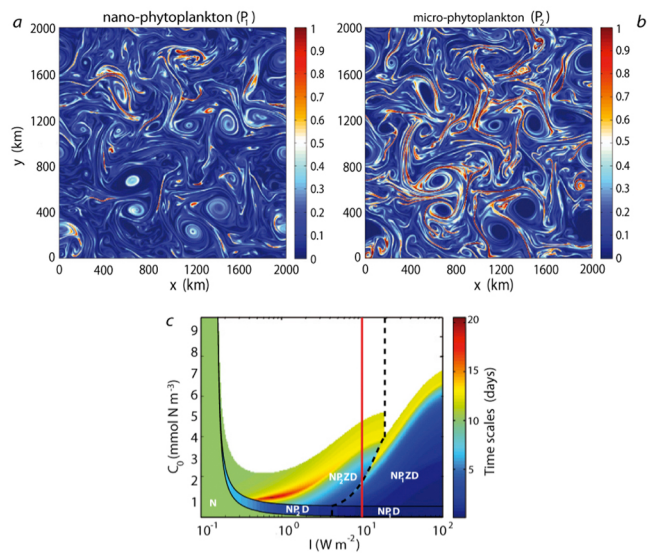
Figure 6. Spatial distribution snapshot of phytoplankton size classes (a) P_1 and (b) P_2 in a submesoscale-resolving model (colour bar in mmol N m^{-3} ). (c) Equilibrium community structure under different total nitrogen ( C_0 ) and irradiance ( I ) conditions (note that irradiance axis is logarithmic). White letters indicate the state variables that exist at equilibrium for the given irradiance and nutrient concentration. Note that P_1 and P_2 do not coexist at equilibrium. Time scale to reach equilibrium (in days) is indicated in colours (white area corresponds to limit cycles at equilibrium). Dashed line separates the two regions in which either P_1 or P_2 exists at equilibrium. Red line indicates the position in the parameter space corresponding to the SQG simulation with a fixed irradiance level of 10 W m^{-2} (adapted from Perruche et al. [2010, 2011]). The coexistence of P_1 and P_2 in the SQG model is due to the perturbations of the ecosystem by mesoscale and submesoscale motions, maintaining the ecosystem out of equilibrium.
