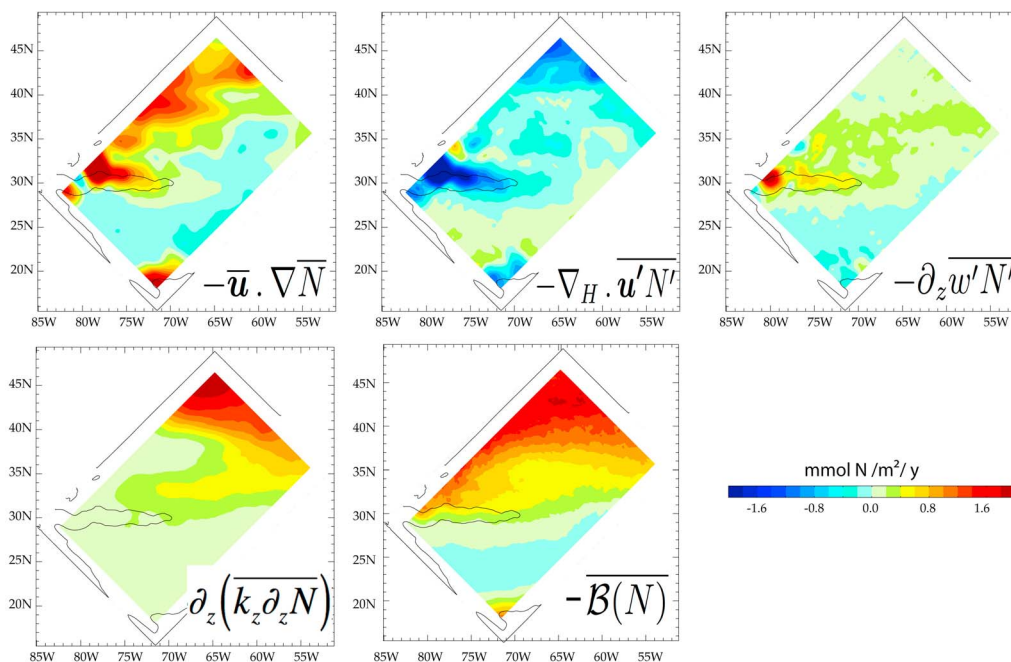
Figure 4. Contribution of all terms in the nitrate ( N = \text{NO}_3 ) equation (equation (1)) from an idealized model simulation representative of the Northwest Atlantic or Northwest Pacific subtropical to subpolar regions. The terms are averaged over the year and over the euphotic depth, as in equation (2). The model is at equilibrium, hence the biological term \int_{1\text{year}} \int_{z=0}^{Z_{\text{eupho}}} \overline{B(N)} dz dt is exactly balanced by the sum of the four physical terms \int_{1\text{year}} \int_{z=0}^{Z_{\text{eupho}}} \left[ -\bar{u} \cdot \nabla \bar{N} - \nabla_H \cdot \overline{u'N'} - \partial_z \overline{w'N'} + \partial_z (k_z \partial_z \bar{N}) \right] dz dt . The black contour shows the annual mean location of the model's idealized Gulf Stream or Kuroshio current. The mean of the fields, denoted with an overbar, is defined in this computation as a coarse-grained running average of 2^\circ width.
