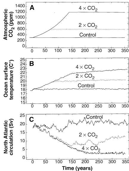
Fig. 1. (A) Atmospheric CO 2 as specified in the control, 2 × CO 2 , and 4 × CO 2 model simulations. (B) Global mean ocean surface temperature simulated by the coupled ocean-atmosphere model. (C) Maximum overturning circulation in the North Atlantic thermohaline cell. Note that the North Atlantic thermohaline cell increases slightly in the control scenario over the time span of the simulation. Manabe and Stouffer did not observe such an increase (5), probably because their initial ocean circulation was different from ours.
