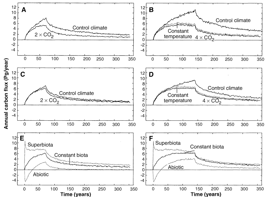
Fig. 2. Annual oceanic uptake of CO 2 . (A) The solubility model with atmospheric CO 2 fixed according to the 2 × CO 2 scenario of Fig. 1A. Two scenarios were run: one used the control climate (the baseline scenario) and the other used the 2 × CO 2 climate. (B) The same as (A) but with CO 2 fixed according to the 4 × CO 2 scenario of Fig. 1A. The constant-temperature scenario allows the ocean circulation to change as in the 4 × CO 2 climate but keeps the temperature used for the carbon chemistry calculations fixed at the initial value. (C) and (D) are analogous to (A) and (B), respectively, but were run in the OBM. (E) and (F) show how the oceanic uptake in the OBM changes if the ocean biology is modified to remove all the nutrients at the surface all the time (the superbiota scenario) or if all organisms die (the abiotic scenario).
