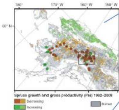
Beck et al. Eco Let. 2011
