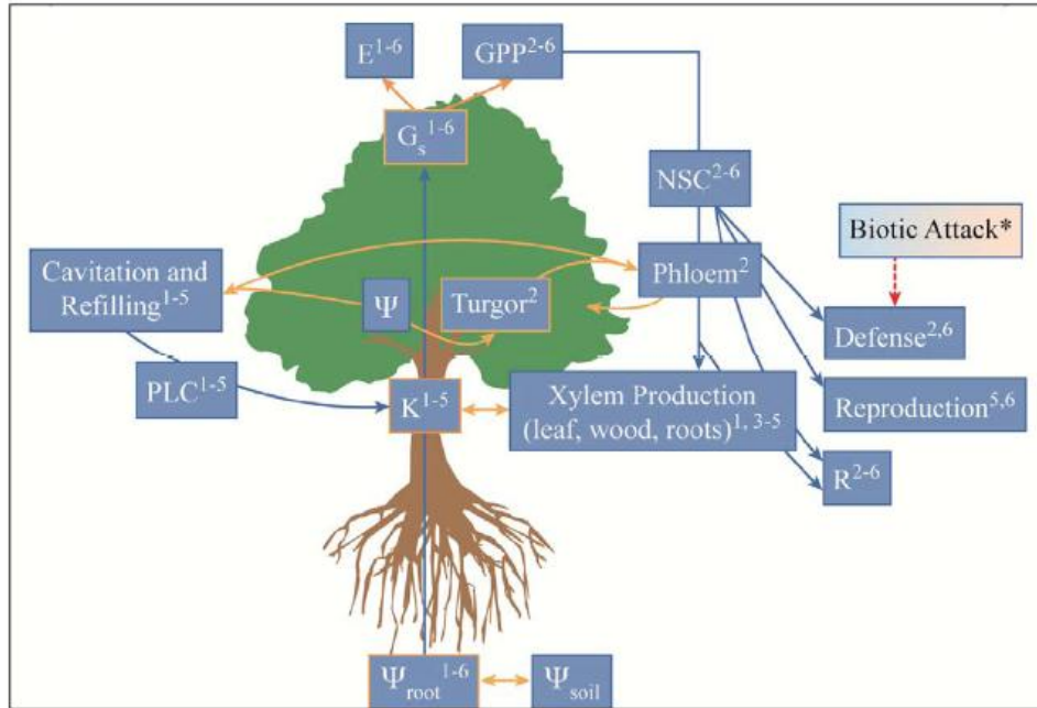
Figure 1. A generalized simulation scheme for modeling plant hydraulic failure, carbon starvation, and their interdependence. The numbers within each box indicate inclusion by the following models: 1 Sperry model, 2 FINNSIM, 3 TREES, 4 MuSICA, 5 ED(X), and 6 CLM(ED). Orange-bordered boxes and orange arrows indicate interdependencies, or bi-directional carbon-water fluxes, that are simulated by the models. Allocation of NSC to defense, reproduction, respiration, and growth are not listed in priority order, because that remains a subject of debate. Abbreviations are canopy transpiration ( E ), canopy-scale stomatal conductance ( G s ), leaf area index ( LAI ), non-structural carbohydrate ( NSC ), hydraulic conductance ( K ), percent loss conductivity ( PLC ) soil and root water potential ( \Psi_{\text{soil}} and \Psi_{\text{root}} ), gross primary production ( GPP ), and autotrophic respiration ( R ). *Biotic attack was not included in any of the models used in this study, but is included to highlight the need for this critical model development (red arrow). Feedbacks between biotic attack and plant physiology are not highlighted here.
