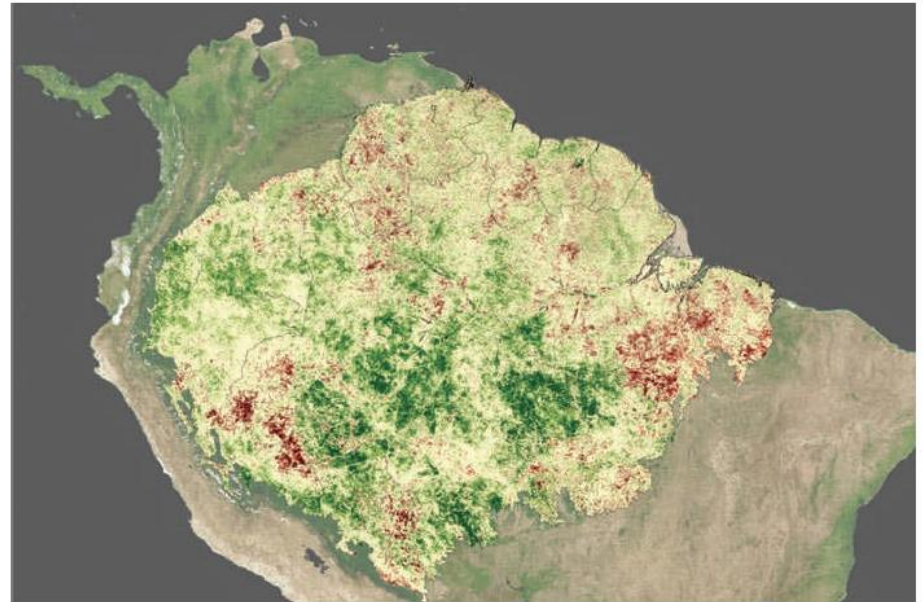
A controversial 2007 study found increased 'greening' in the Amazon rainforest during a drought in 2005.
