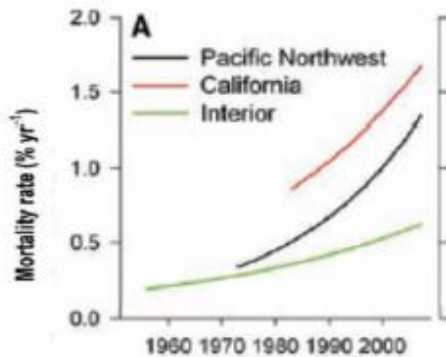
Van Mantgem et al. Science 2011
