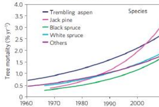
Peng et al. Nature Climate Change 2011
