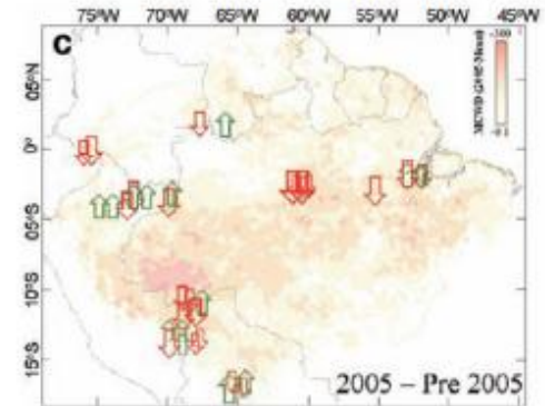
Phillips et al. Science 2009
