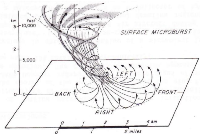
Fujita, 1985
