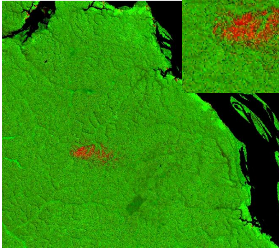
Landsat sub-image from 2001 image – west bank of Rio Negro north of Manaus
