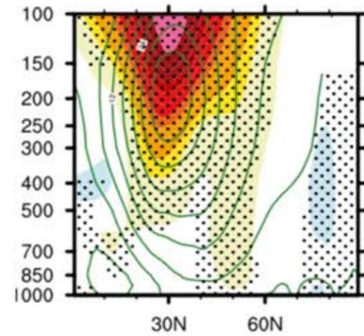
GHG Forcing without Ice Loss
