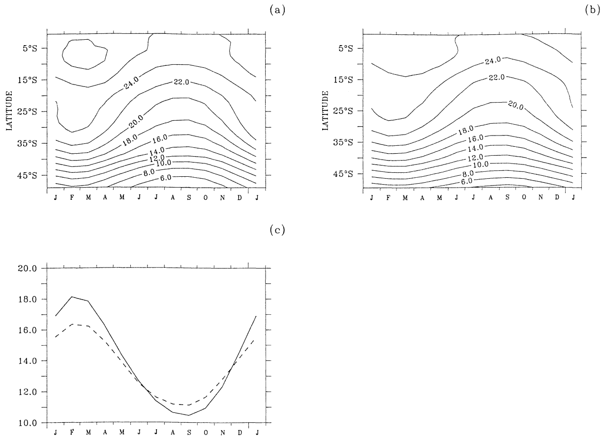
Figure 8. Comparison of the annual cycle of SST, zonally averaged between 65°W and 15°E, for (a) the CSM climatology and (b) the Reynolds and Smith [1994] climatology. Contour interval is 2°C. Comparison of (c) the zonally averaged SST (°C) climatologies at 40°S; CSM is denoted by the solid line and Reynolds and Smith [1994] by the dashed line.
