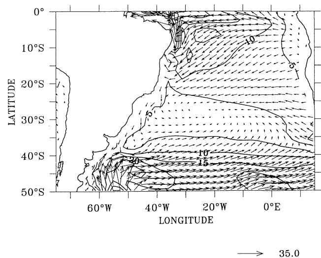
Figure 1. Climate System Model (CSM) annual mean surface currents. Maximum vector length is 35 \text{ cm s}^{-1} ; velocity magnitude contour interval is 5 \text{ cm s}^{-1} .
